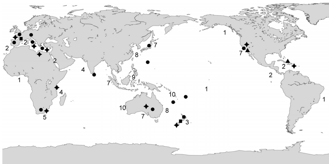
FIGURE 1. Worldwide distribution of living and fossil abalone. Numerals indicate approximate number of living species in each region. Fossil distribution represent by symbols ▲ = Cretaceous, ■ = Paleogene, ● = Neogene, ◆ = Pleistocene. Distributional data from Geiger (1998, 2000); fossil data from Geiger and Groves (1999).
