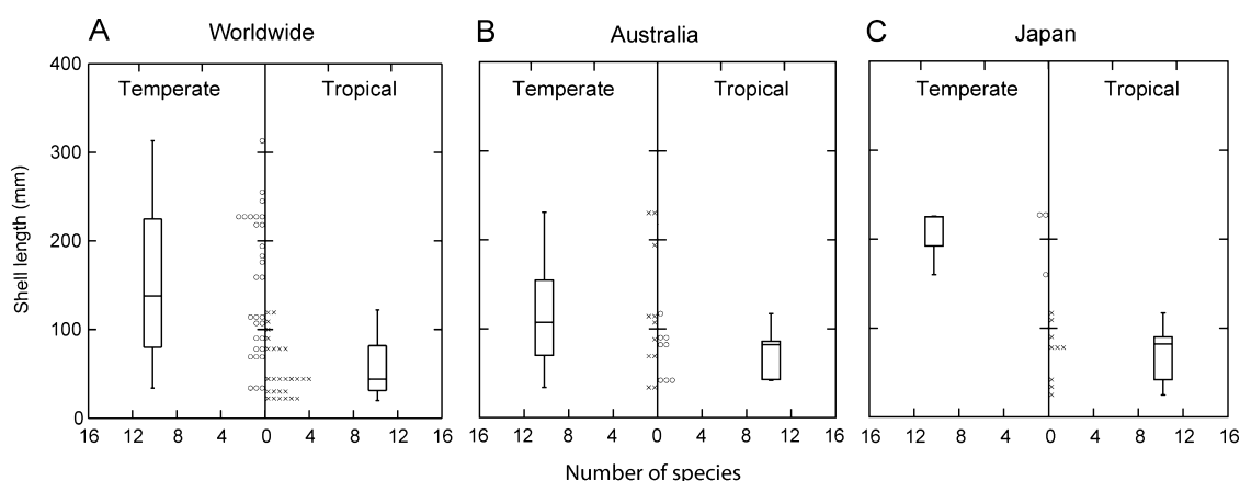
FIGURE 2. Size distributions of temperate and tropical abalones. A, Worldwide fauna. B, Latitudinal gradient from north (tropical) to south (temperate) along the western and eastern coasts of Australia. C, Latitudinal gradient from north (temperate) to south (tropical) along the western and eastern coasts of Japan. Box plots display sample means and quartiles. Two-sample t -test probabilities (Bonferroni adjusted—all corrected on the basis of same number of tests) on size grouped by regions: tropical vs. temperate ( t_{55} = 5.881 , p < 0.0001 ); Japan tropical vs. Japan temperate ( t_{10} = 5.821 ; p < 0.0001 ); Australian tropical vs. Australian temperate ( t_{17} = 1.674 ; p = 0.112 ). Size data from Lindberg (1992), Geiger (1998, 2000), and Hutsell et al. (1999); distributional data from Geiger (2000).
