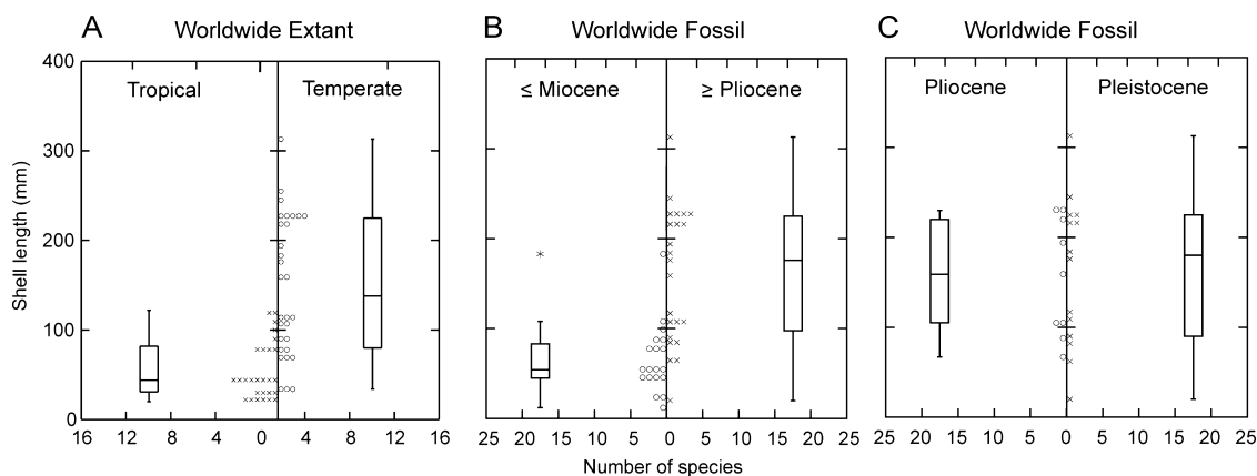
FIGURE 4. Size distributions of living and extinct abalone taxa. A, Living taxa. B, Pre-Pliocene taxa vs. post Miocene taxa. C, Pliocene taxa vs. Pleistocene taxa. Box plots display sample mean and quartiles; * = outliers. See Figure 2 for data sources for living taxa. Fossil occurrences for Haliotis species from Geiger and Groves (1999).
