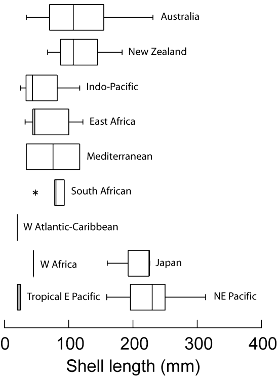
FIGURE 3. Size distributions of living abalone taxa by regions. Box plots display sample medians and quartiles; * = outliers. Size data from Lindberg (1992), Geiger (1998, 2000), and Hutsell et al. (1999); distributional data from Geiger (2000).
